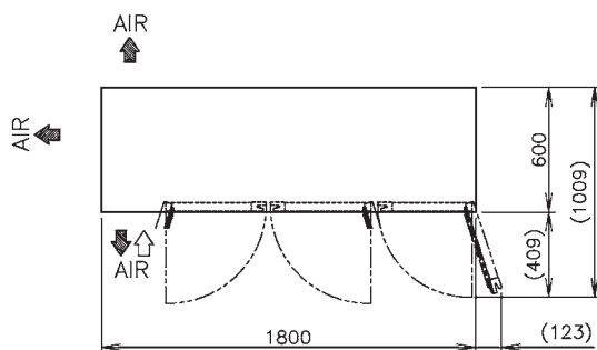
VIEW A(1/10)
